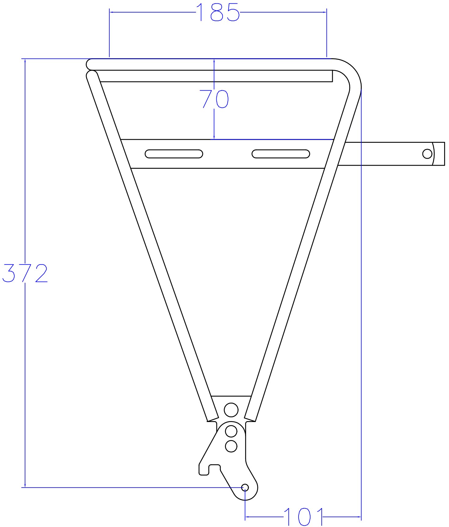
Old Man Mountain Sherpa front 26"
